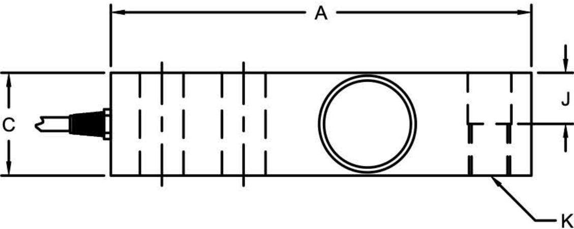
CG-23-SS THREADED LOAD HOLE
