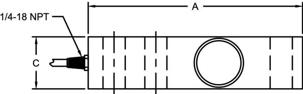
CG-23-SS-1 NON-THREADED LOAD HOLE
